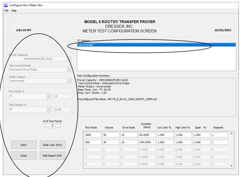
Figure 1.18 Example - Prover Configuration screen for Model 5 Prover software
