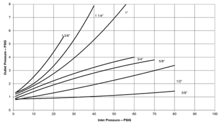
B-38R Relief Curves – Blocked Per Orifice 14" w.c. Set Point
