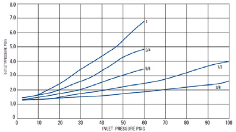
B38 IM RELIEF CURVES - BLOCKED PER ORIFICE 1 PSIG SET POINT
