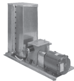
Single headed chemical injector with 10 gallon SS tank. Weight 105 pounds.
