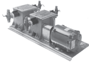
Double headed chemical injector with two 5 gallon SS tanks. Weight 110 pounds.
