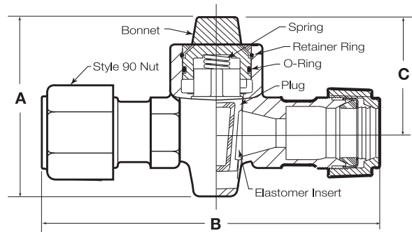
Style 175 Meter Valve with Style 90 Compression Ends
