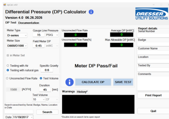
Figure 1 – Low Flow Meter Test Screen
