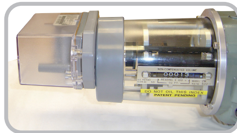
AMR Adapter and ERT installed on a Dresser meter (top inlet meter installation shown)
