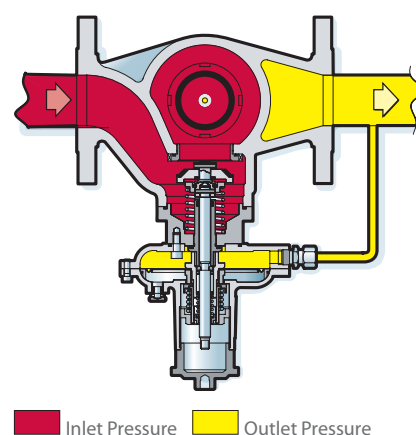
Operational Diagram
