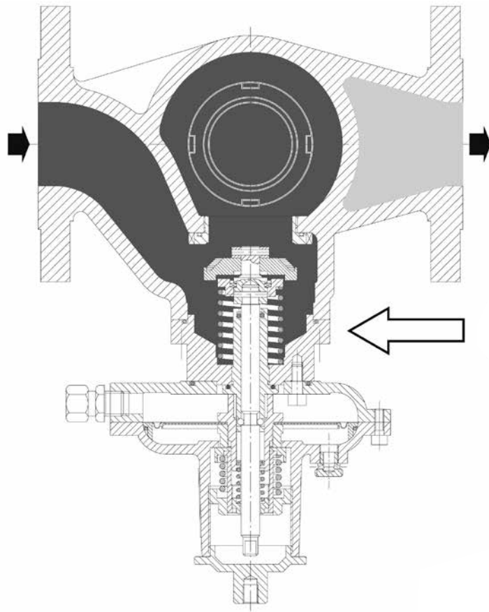
Built-in SSV 8500 by RB 4000 Regulator
