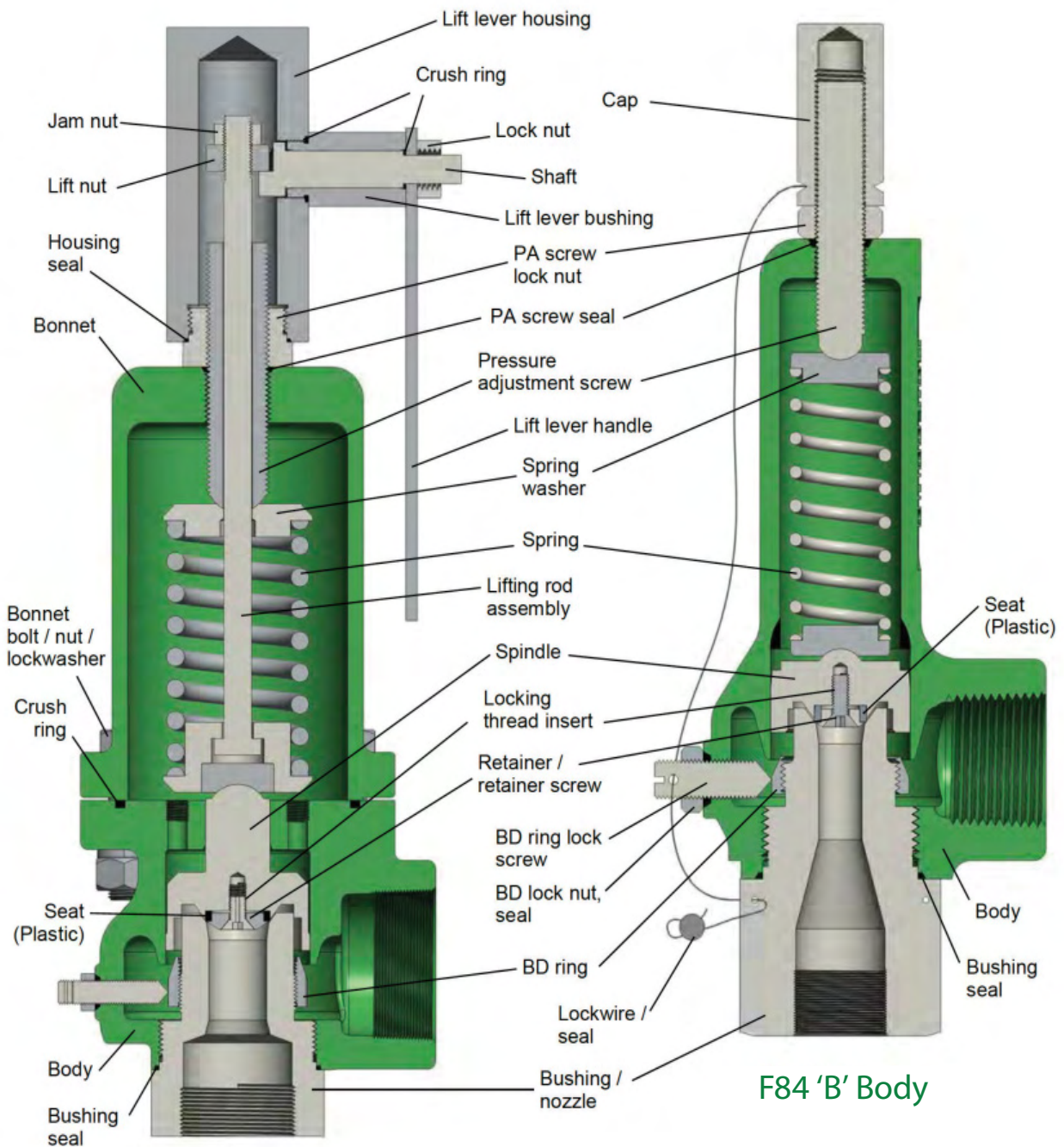
F84 'C'/'D'/'E' Body with Lift Lever
