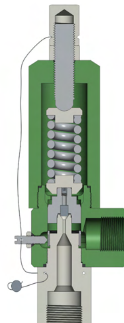
F85M 'M' (Micro) Body - Standard F85M-3 w/ NPT connections shown
