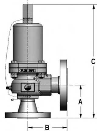
C, D, E Body - Bolted Bonnet (Lift lever shown)
