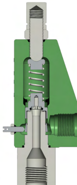
F85M 'M' (Micro) Body - HP Block F85M-4 w/ SAE AS5202 connections shown
